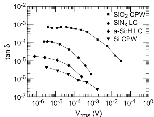
FIG. 1. Loss tangent after adjusting for the electrical loading. Data labeled \text{SiO}_2 and Si correspond to 300 nm plasma-enhanced chemical vapor deposition (PECVD) \text{SiO}_2 on single-crystal Si, and 100 \Omega -cm single-crystal Si, respectively. All resonators had Al electrodes. Measurements made with T \leq 100 mK.
