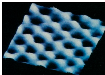
Figure 3. Crystal lattice of Muscovite mica imaged by atomic force microscopy (AFM), showing locations of recessed hydroxyl (OH) and ionized hydroxyl (O - ) groups, as depressions (dark spots) on the mica surface. Image size is 2.6 nm × 2.6 nm. Modified from [58].
