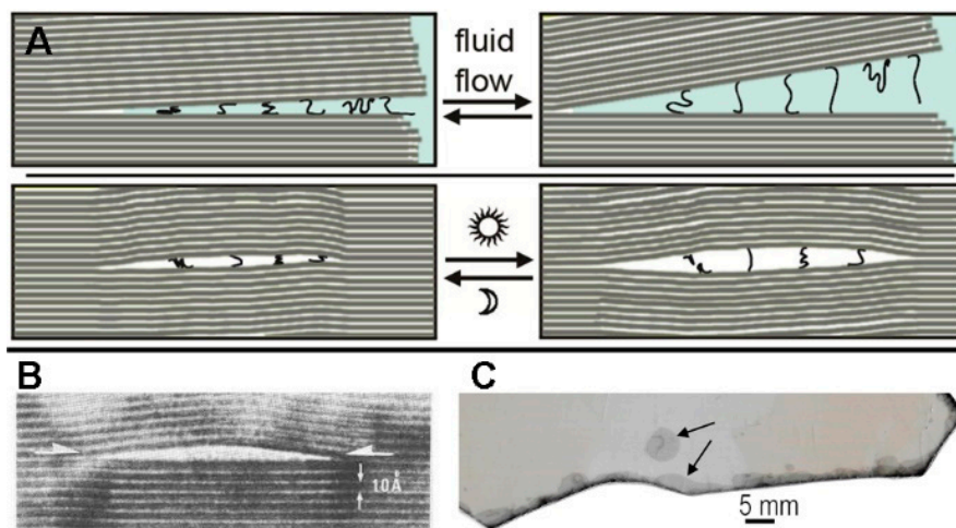
Figure 2. (A) Diagram of mechanical forces between biotite mica sheets, stretching and compressing polymers, due to: (Upper panels) water flow at the edges of the biotite sheets, and (Lower panels) heat pumps in a biotite bubble. (B) Biotite bubble imaged by HRTEM (high-resolution transmission electron microscopy). The thickness of a single biotite sheet is 1 nm (10 Angstroms) [55]. (C) Top view of a bubble in Muscovite mica (upper arrow) and of sheet separation at the edges of the mica sheet (bottom arrow). Bubbles are common even in ‘high grade’ micas. Biotite is now the preferred mica, for life’s origins between mica sheets [56,57].
