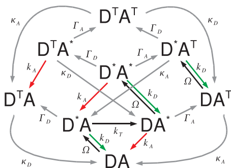
FIG. 2. Kinetic scheme for a nine-state model including donor and acceptor triplet states. Here, \rho_A = k_A(P_{DA^*}^{ss} + P_{D^*A^*}^{ss} + P_{D^*A}^{ss} + P_{D^*A^*}^{ss}) and \rho_D = k_D(P_{D^*A^*}^{ss} + P_{D^*A}^{ss} + P_{D^*A^*}^{ss}) . Rate constants not appearing in Fig. 1 are for intersystem crossing to ( \Gamma_D, \Gamma_A ) and from ( \kappa_D, \kappa_A ) the triplet states.
