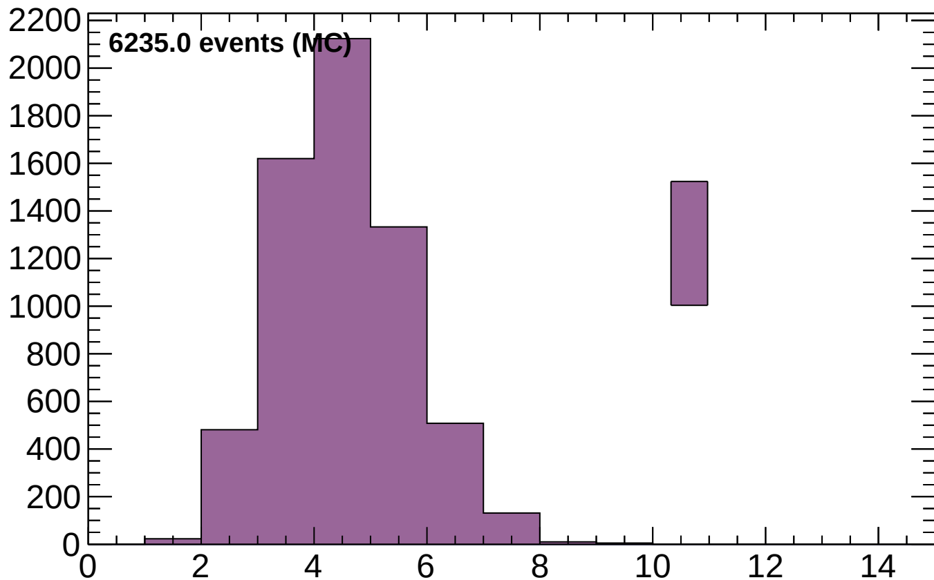
number of good reco jets
