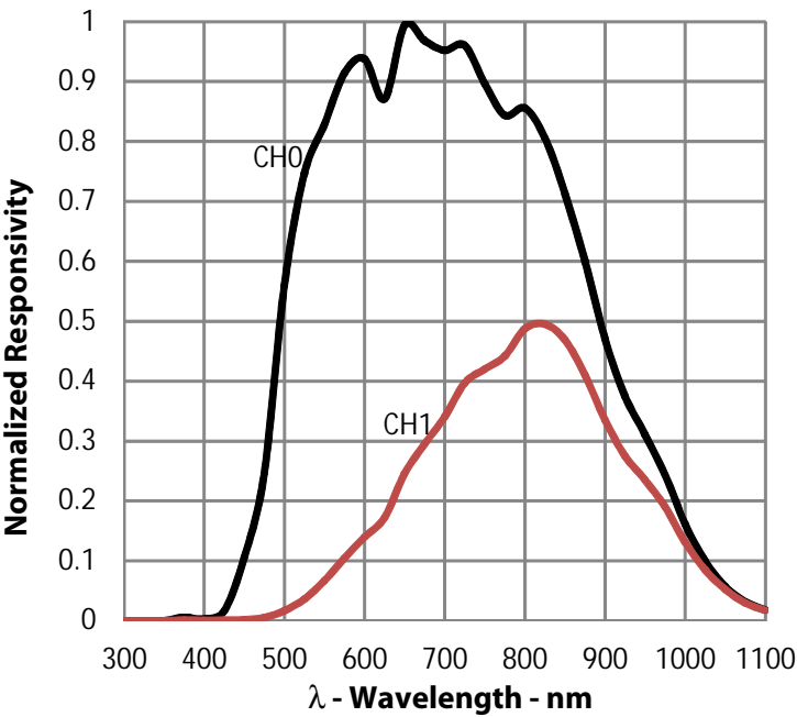
Figure 11: Spectral Responsivity
