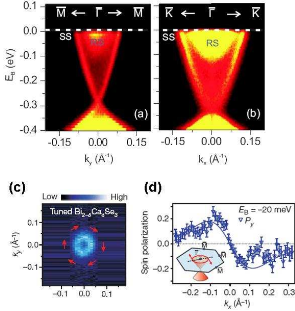
FIG. 25 ARPES data for the dispersion of the surface states of \text{Bi}_2\text{Se}_3 , along directions (a) \bar{\Gamma} - \text{M} and (b) \bar{\Gamma} - \bar{\text{K}} in the surface Brillouin zone. Spin-resolved ARPES data is shown along \bar{\Gamma} - \text{M} for a fixed energy in (d), from which the spin polarization in momentum space (c) can be extracted. From Xia et al. , 2009 and Hsieh et al. , 2009.
