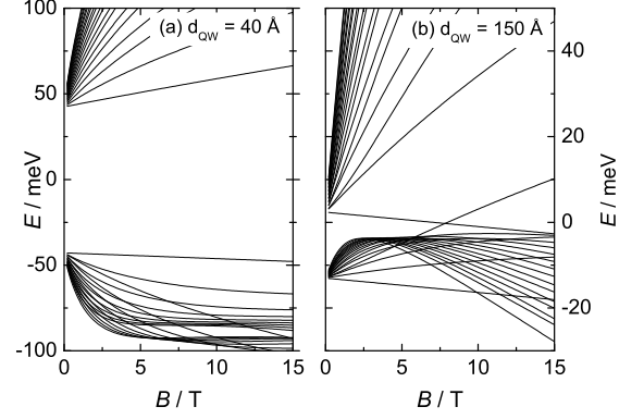
FIG. 11 Landau level dispersion for quantum well thicknesses of (a) 4.0 nm, (b) 15.0 nm. The qualitative behavior is indicative for samples with (a) normal and (b) inverted band structure. From König et al. , 2008.
