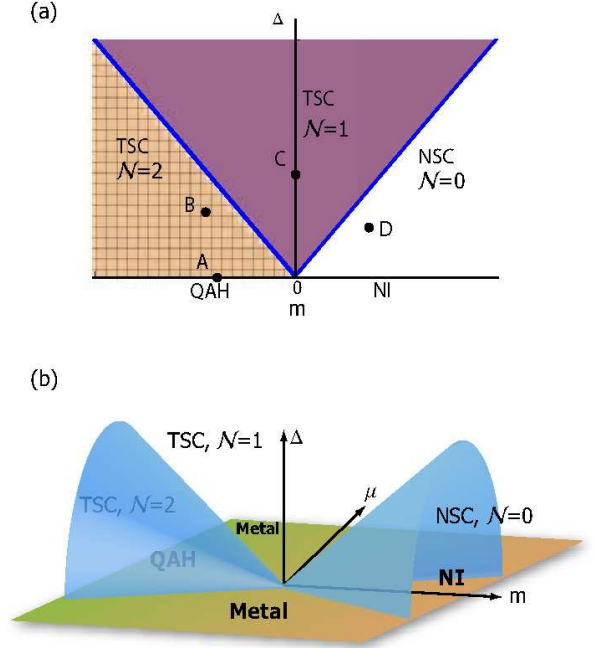
FIG. 43 (a) Phase diagram of the QAH-superconductor hybrid system for \mu = 0 . m is the mass parameter, \Delta is the magnitude of the superconducting gap, and N is the Chern number of the superconductor, which is equal to the number of chiral Majorana edge modes. (b) Phase diagram for finite \mu , shown only for \Delta \geq 0 . The QAH, normal insulator (NI) and metallic (Metal) phases are well-defined only for \Delta = 0 . From Qi et al. , 2010.
