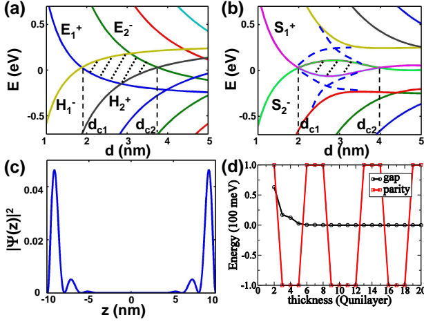
FIG. 21 Energy levels versus quantum well thickness for (a) A_1 = 0 eV·Å, (b) A_1 = 1.1 eV·Å. Other parameters are taken from Zhang et al. , 2009. Shaded regions indicate the QSH regime. The blue dashed line in (b) shows how the crossing between |E_1(H_1)\rangle and |H_2(E_2)\rangle evolves into an anti-crossing when A_1 \neq 0 . (c) Probability density in the state |S_1^+\rangle (same for |S_2^-\rangle ) for A_1 = 1.1 eV·Å and d = 20 nm. (d) Band gap and total parity from ab initio calculations on Bi 2 Se 3 , plotted as a function of the number of quintuple layers. From Liu et al. , 2010.
