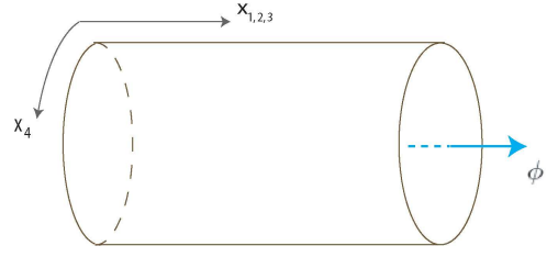
FIG. 35 Dimensional reduction from (4 + 1)\text{D} to (3 + 1)\text{D} . The x_4 direction is compactified into a small circle, with a finite flux \phi threading through the circle due to the gauge field A_4 . To preserve TR symmetry, the total flux can be either 0 or \pi , resulting in a \mathbb{Z}_2 classification of 3D topological insulators.
