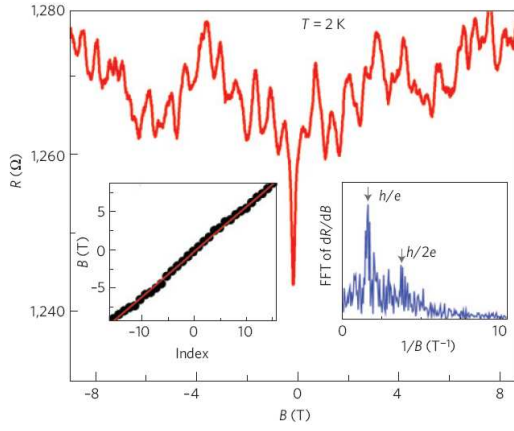
FIG. 32 Magnetoresistance for fields up to \pm 9 T. Left inset: magnetic fields at which well-developed resistance minima are observed. Right inset: fast Fourier transform of the resistance derivative dR/dB , where peaks correspond to hc/e and hc/2e oscillations are labeled. From Peng et al. , 2010.
