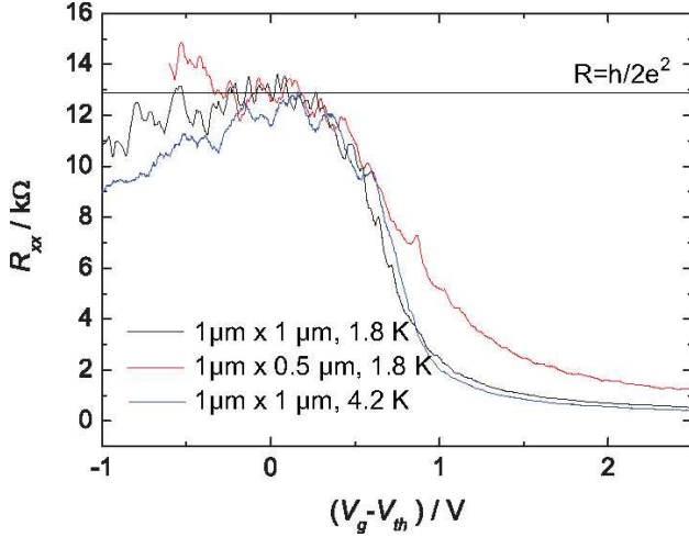
FIG. 14 Longitudinal resistance as a function of gate voltage for two devices with L = 1 \text{ }\mu\text{m} . The width W is 1 \text{ }\mu\text{m} [solid (black) and dotted (blue)] and 0.5 \text{ }\mu\text{m} [dashed (red)]. The solid and dashed traces were obtained at a temperature of 1.8 \text{ K} , and the dotted one at 4.2 \text{ K} . From König et al. , 2008.
