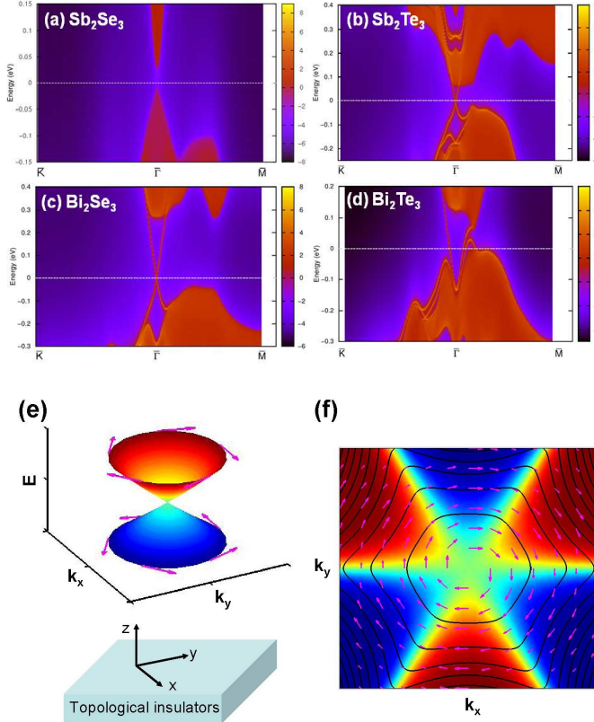
FIG. 20 (a)-(d) Energy and momentum dependence of the local density of states for the Bi 2 Se 3 family of materials on the [111] surface. A warmer color represents a higher local density of states. Red regions indicate bulk energy bands and blue regions indicate a bulk energy gap. The surface states can be clearly seen around \Gamma point as red lines dispersing inside the bulk gap. (e) Spin polarization of the surface states on the top surface, where the z direction is the surface normal, pointing outwards. Adapted from Zhang et al. , 2009 and Liu et al. , 2010.
