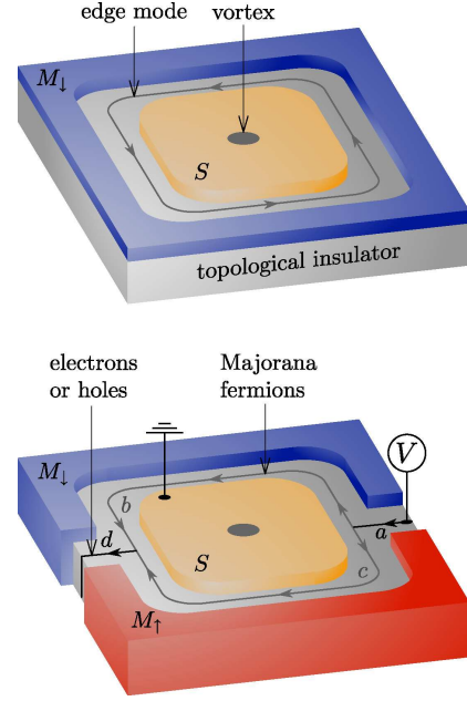
FIG. 44 3D topological insulator in proximity to ferromagnets with opposite polarization ( M_\uparrow and M_\downarrow ) and to a superconductor ( S ). The top panel shows a single chiral Majorana mode along the edge between superconductor and ferromagnet. This mode is electrically neutral, and therefore cannot be detected electrically. The Mach-Zehnder interferometer in the bottom panel converts a charged current along the domain wall into a neutral current along the superconductor (and vice versa). This allows electrical detection of the parity of the number of enclosed vortices/flux quanta. From Akhmerov et al. , 2009.
