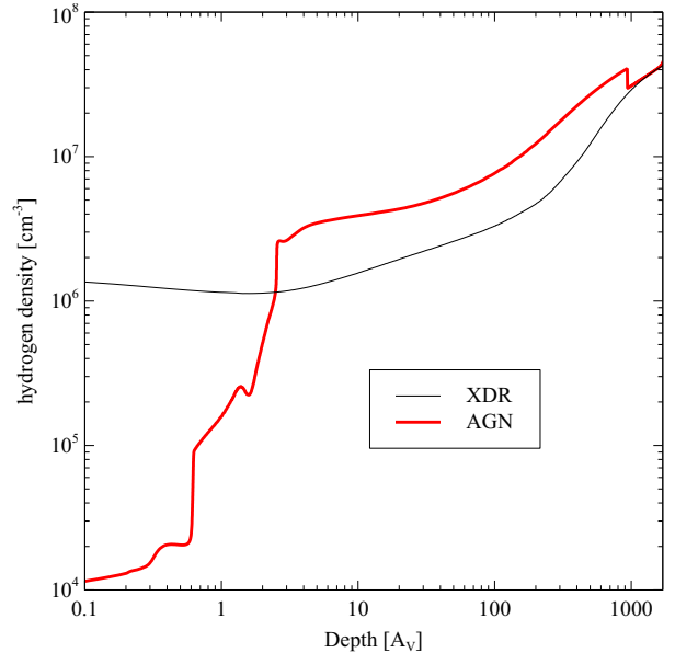
Fig. 12. The hydrogen density is shown for the XDR and AGN clouds.
