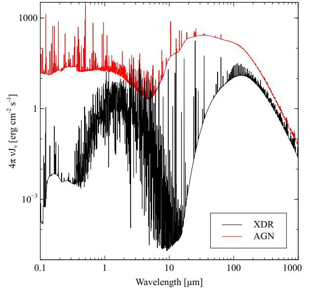
Fig. 16. The spectra emitted by the XDR and AGN simulations are shown.
