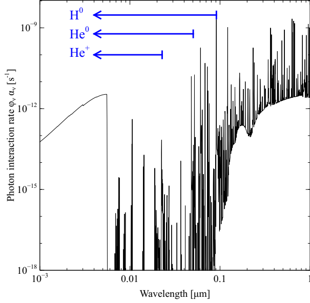
Fig. 8. This shows a small portion of the radiation field around wavelengths capable of ionizing H and He. The horizontal lines indicate thresholds for photoionization of H^0 , He^0 , and He^+ .
