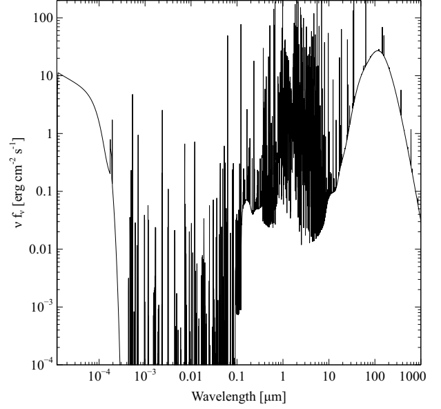
Fig. 9. The spectrum emergent from the XDR2 cloud. Thermal dust emission dominates in the IR while the incident XDR continuum dominates in the X-ray. A rich UV, FUV, and EUV spectrum is emitted by atoms and ions within the gas.
