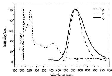
Figure 4. PL, EL and absorption spectra of Al(Saph-q). a) absorption spectrum; b) PL spectrum; c) EL spectrum.
