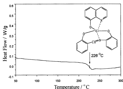
Figure 1. The molecular structure and DSC chart of (Al(Saph-q)).
